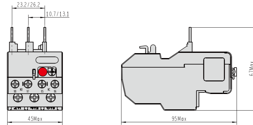
Overall Dimensional Drawing of HDR3s-25/Z
