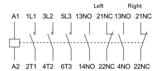
DOL Control
