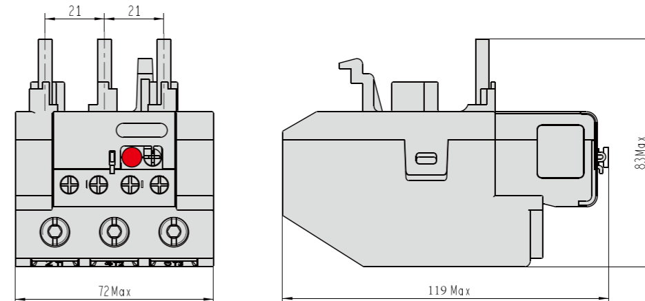
Overall Dimensional Drawing of HDR3s-93/Z
